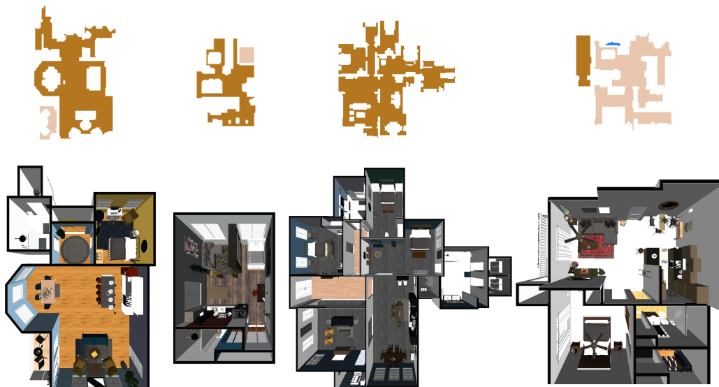
Figure 8: Visualization of the navigable geometry (top row) and top-down views of example scenes from the Habitat Synthetic Scenes Dataset (HSSD) [19]. We use the computed navigable area to efficiently generate a large number of episodes for the Open-Vocabulary Mobile Manipulation task. Object placement positions are sampled to be near navigable areas of the map, atop one of a large variety of different receptacles, such that the robot can reach them.
